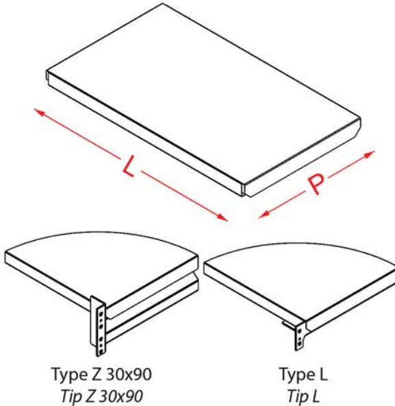
Light Duty Rack Metal Shelf (Push Outside) Hafif Rack Tabla (Dıştan Basma)
