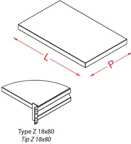
Light Duty Rack Metal Shelf (Push Inside) Hafif Rack Tabla (İçe Basma)
