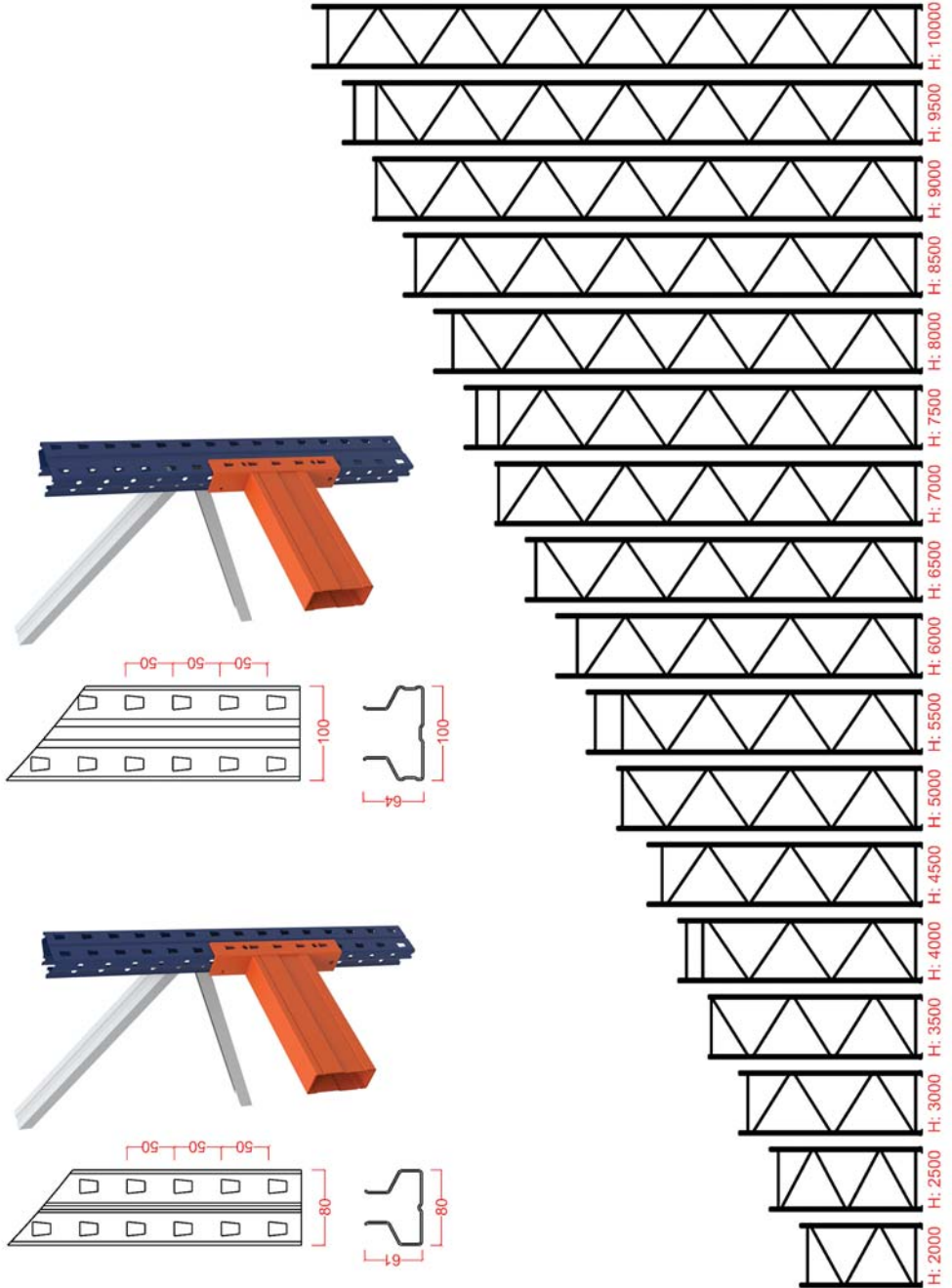
Heavy Duty Rack Frame Leg Ağır Rack Ayak
