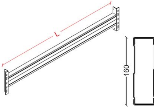
Heavy Duty Rack CC Traverses Ağır Rack CC Travers
