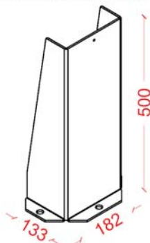
Frame Leg Base Protector U Barrier Ayak Muhafaza U Bariyeri
