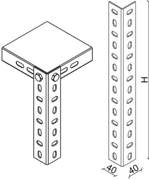
Steel Shelf Upright (40*40) Çelik Raf Profil (40*40)
