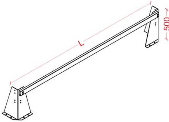
Frame Leg Base Protector Barrier (Single Profile) Ayak Muhafaza Bariyeri (Tek Profilli)
