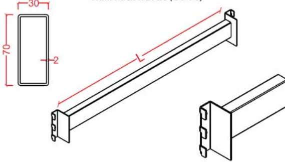
Light Duty Rack Traverses (30*70) Hafif Rack Travers (30*70)
