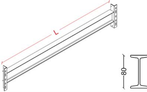
Heavy Duty Rack NPI Traverses Ağır Rack NPI Travers
