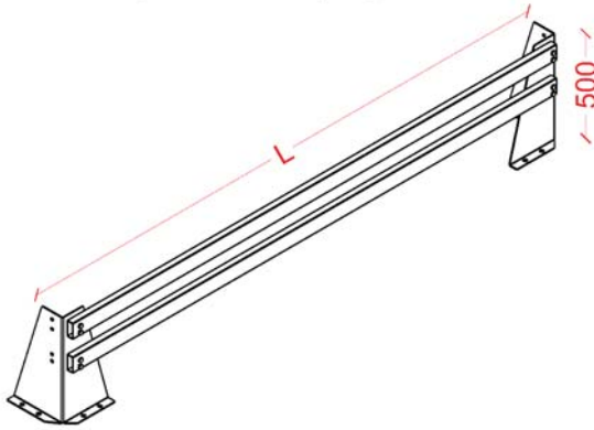
Frame Leg Base Protector Barrier (Double Profile) Ayak Muhafaza Bariyeri (Çift Profilli)
