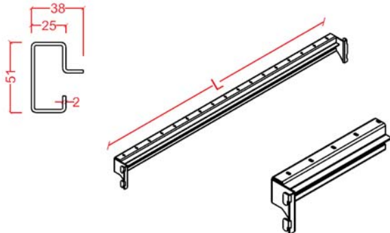
Light Duty Rack Traverses (Ada) Hafif Rack Travers (Ada)
