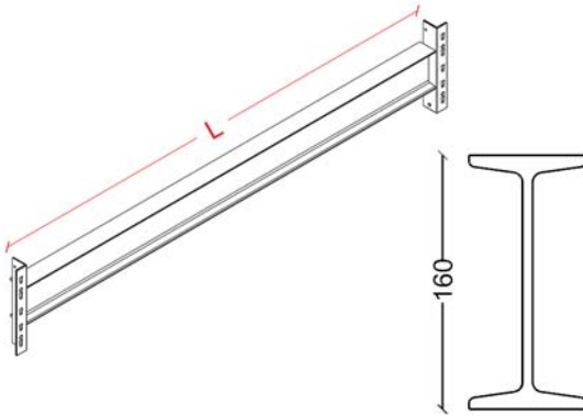
Heavy Duty Rack NPI Traverses Ağır Rack NPI Travers
