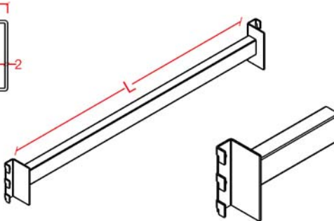
Light Duty Rack Traverses (30*50) Hafif Rack Travers (30*50)
