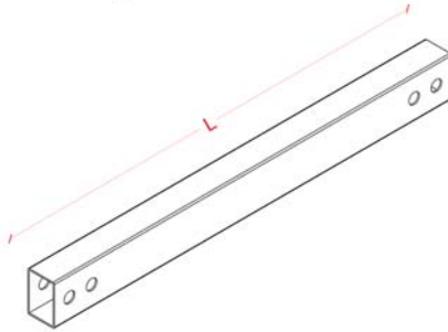
Heavy Duty Rack Elongation Profile Ağır Rack Gerdirme Profili
