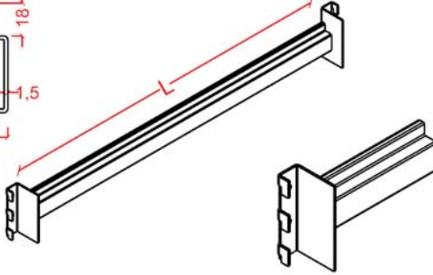
Light Duty Rack Traverses (Type L) Hafif Rack Travers (Tip L)
