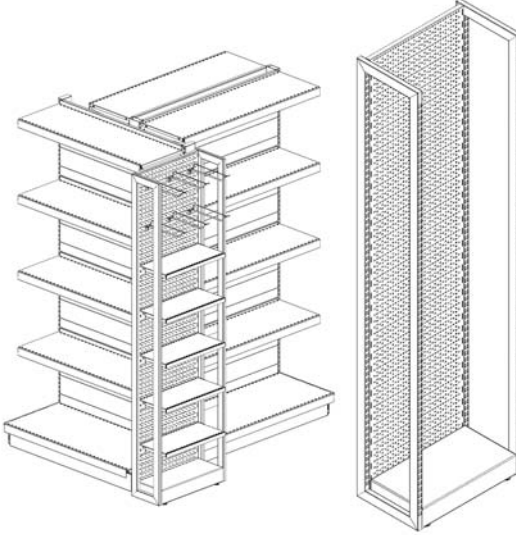
Gondola Side Stand with Profile AP - Main Frame Gondol Yan Stand Profilli AP - Gövde
