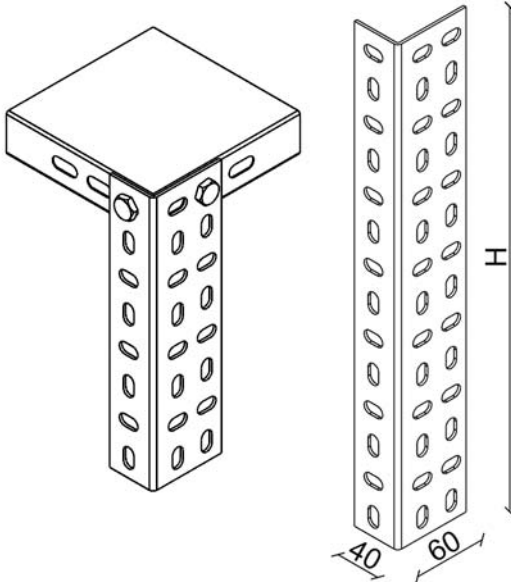
Steel Shelf Upright (40*60) Çelik Raf Profil (40*60)
