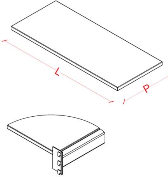
Light Duty Rack Metal Shelf (Push Inside) Hafif Rack Tabla (İçe Basma)
