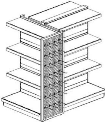
Promotion Cover for Gondola End Unit - DP Gondol Başı Aksiyon Kapama - DP
